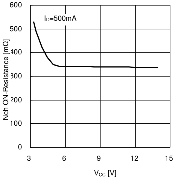
Figure 12. Nch FET ON-Resistance vs V CC
