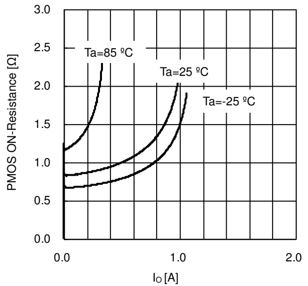
Figure 15. Pch FET ON-Resistance vs I O (V CC =3.5V)
